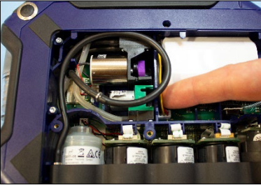
Fig. 76: Pulling out the battery plug
