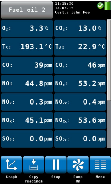
Fig. 18: Display details
