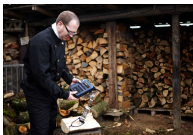
Fig. 46: Wood moisture measurement with Probe Wohler HBF 420.
