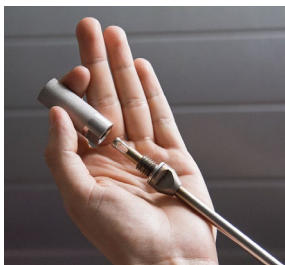
Fig. 9: Flue gas probe 1,000 mm with sinter filter
